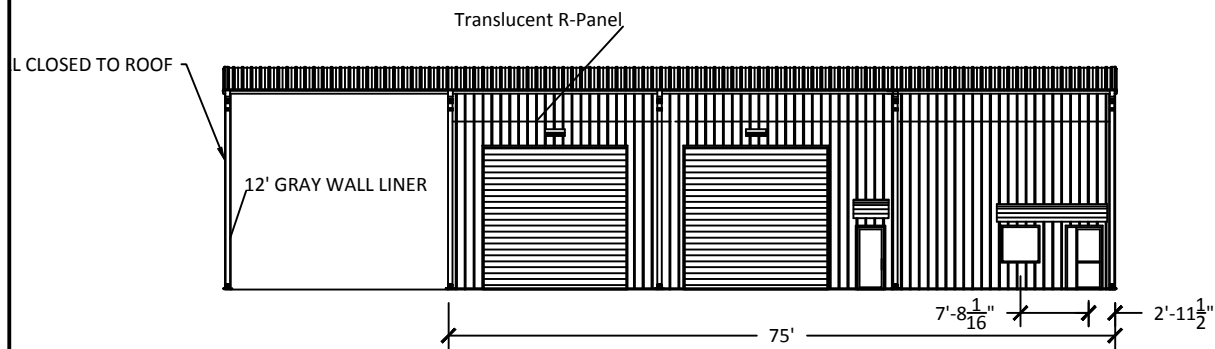
South Elevation
