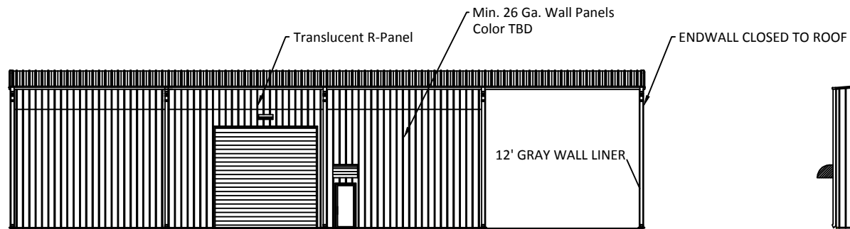
North Elevation
